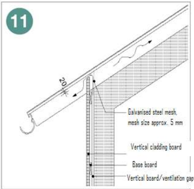
11 Connection of vertical cladding to the eaves. If the underside of the eaves is left open, the upper ends of the vertical boards must be finished with care.
